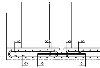
SECTION 1-1 SCALE 1:50
